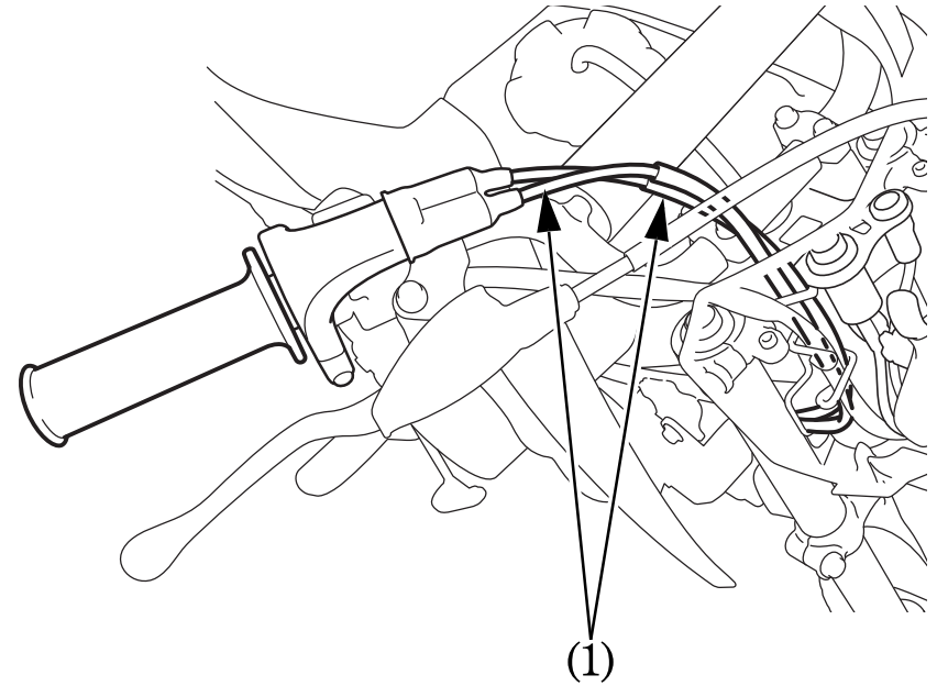
(1) Throttle cables
