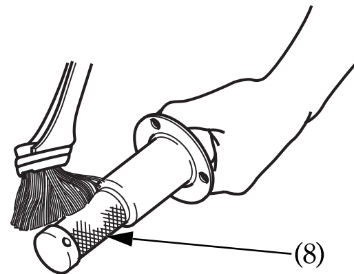
(8) spark arrester screen
