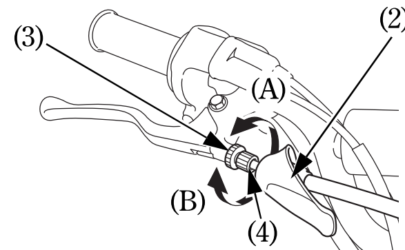
(2) Dust cover
