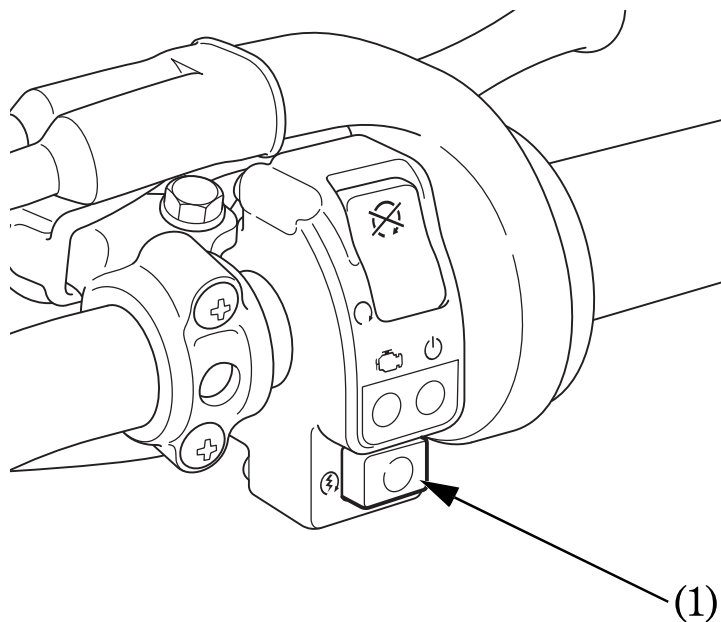
(1) Start button
