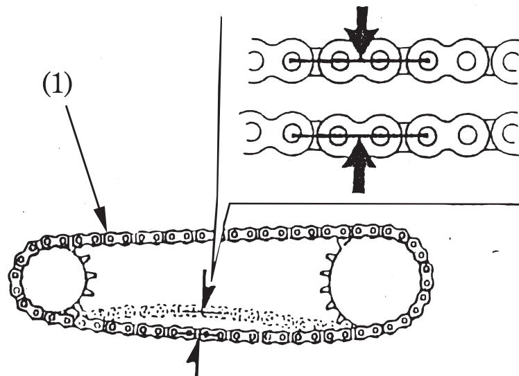
(1) Drive chain
