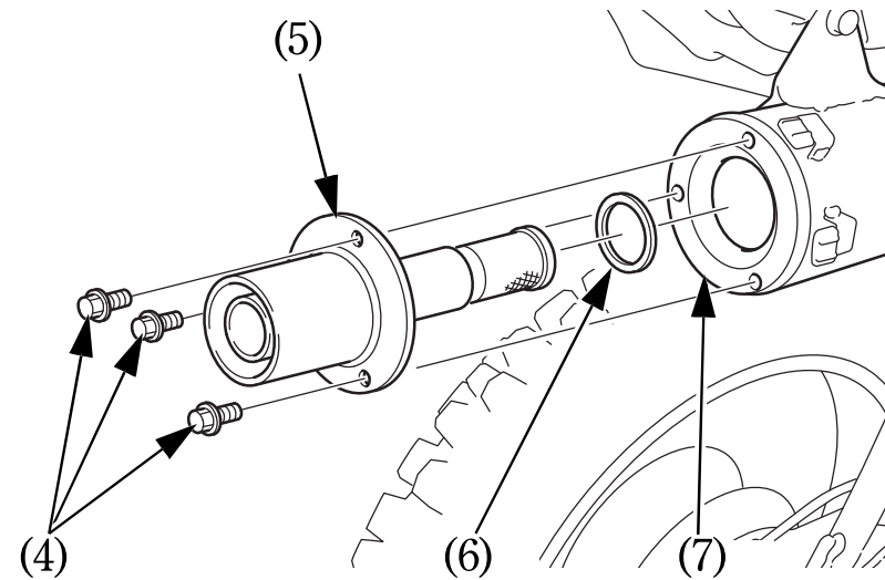
(4) Bolts (5) Spark arrester
