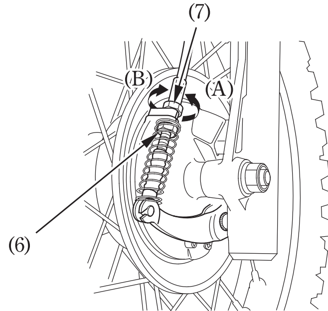
(6) Lock nut (7) Adjusting nut
