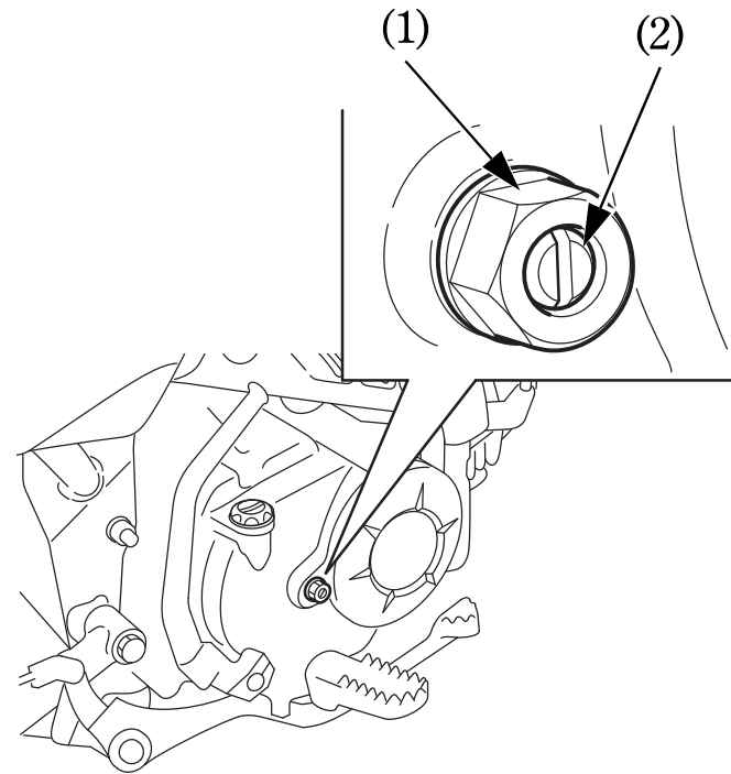
(1) Lock nut
