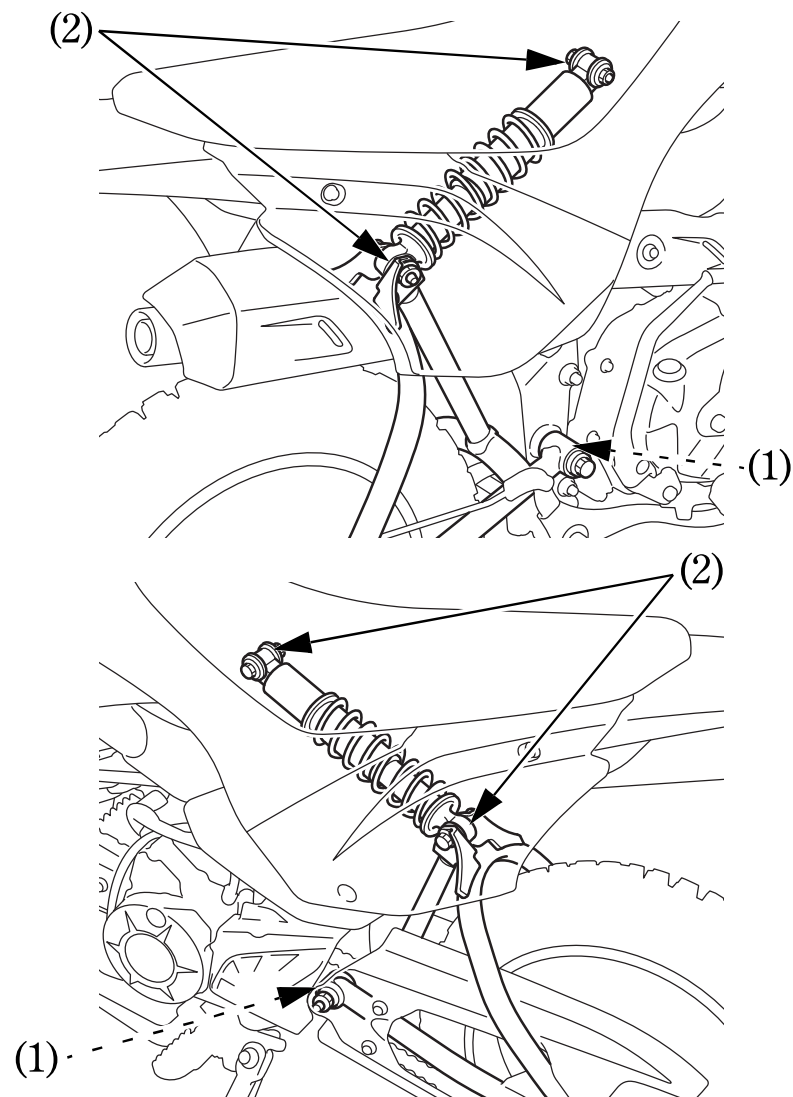
(1) Bushings
