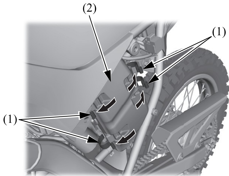
(1) Retainer clips (2) Air cleaner housing cover
