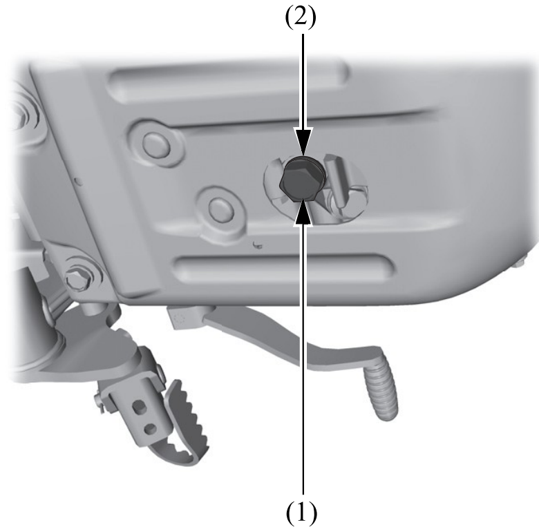
(1) Oil drain bolt
