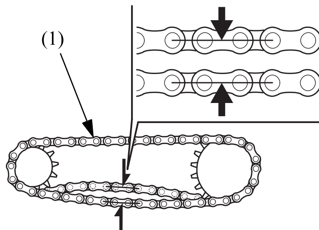
(1) Drive chain
