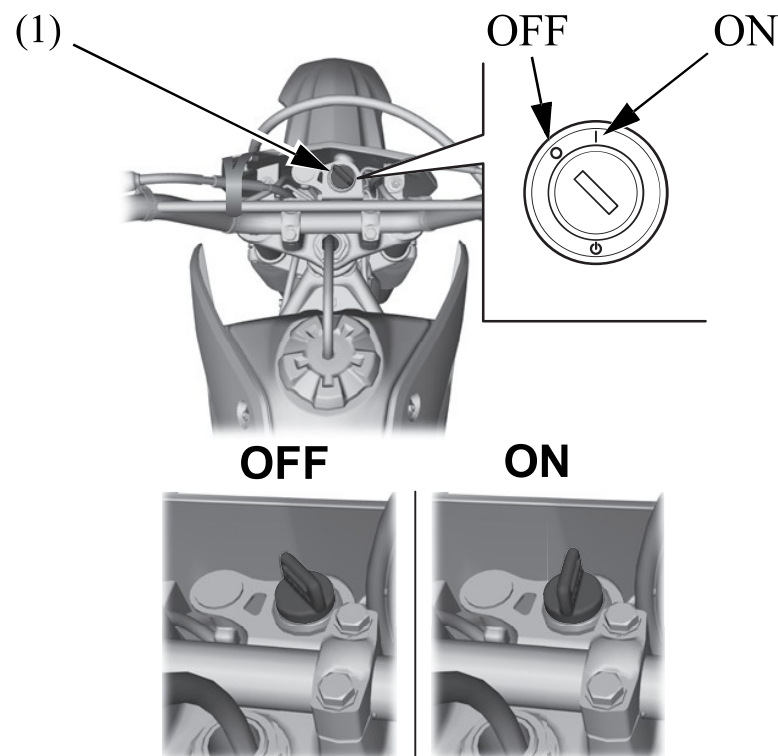
(1) Ignition switch
